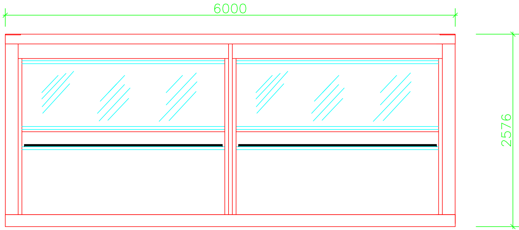
ALZADO PRINCIPAL
